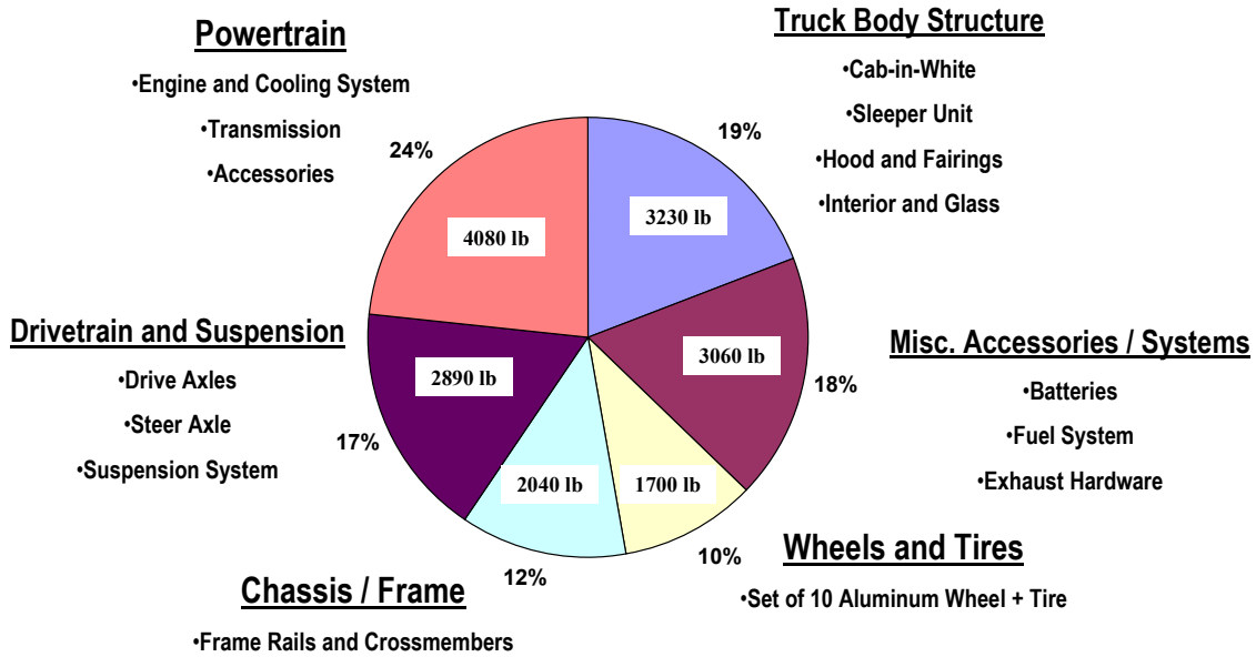
Figure 3. Weight allocation of Class 8 tractor with raised roof sleeper.
