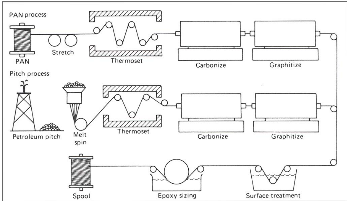
Figure 4. Carbon fiber manufacturing steps.
