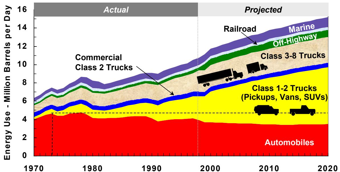
Figure 1: Growth of US surface transportation fuel consumption
