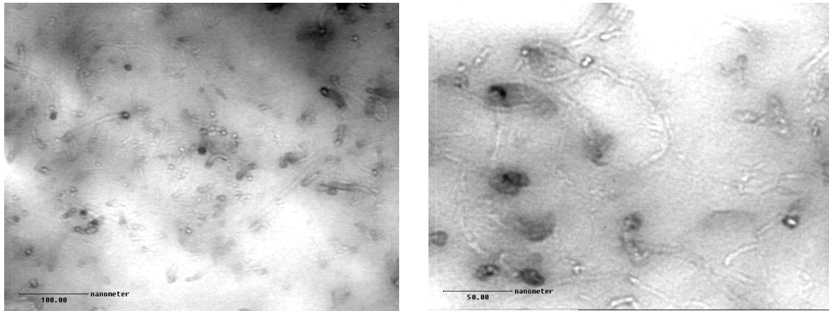
Figure 7. Transmission Electron Micrograph of Ultramicrotomed Section of Nanotube-filled Injection Molded Bar
